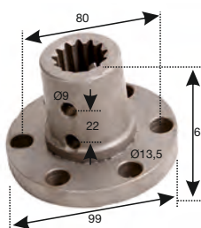
Allradflansch 6-Loch
